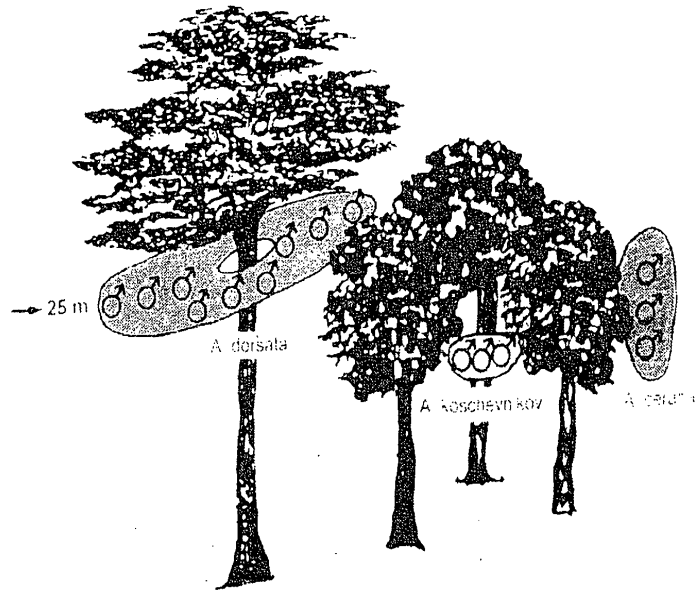
Fig. 1: Drone congregation areas in Sabah (Borneo). A. dorsata drones congregated directly under the canopy of high emergent trees. A. koschevnikovi drones congregated under the thick cover of branches and trees. A. cerana drones remained near the branches of neighbouring vegetation. All three drone congregation areas were within a distance of 30 m. ♂ Spaces occupied by drone flight.
