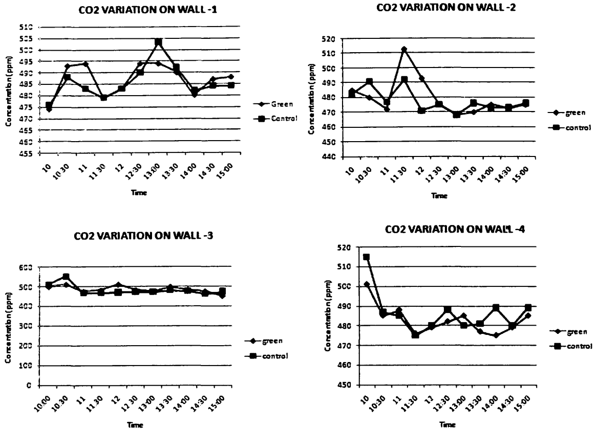
Figure 5 Variation of Carbon dioxide over with time of the day for green walls with different species 1- Tradescathus spathacea , 2- Xiphidium caeruleum , 3- Sansevieria trifasciata , 4- Peperomia obtusifolia
