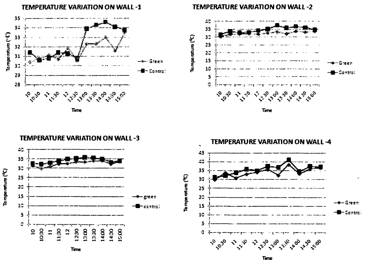
Figure 3 Variation of Temperature over with time of the day for green walls with different species 1- Tradescathus spathacea , 2- Xiphidium caeruleum , 3- Sansevieria trifasciata , 4- Peperomia obtusifolia
