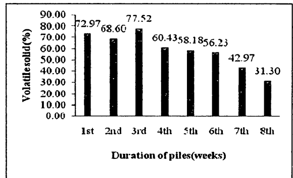
Figure 7: Variation of percent volatile solid content of the composting pile with time
