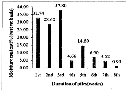
Figure 6: Variation of percent moisture content of the composting pile with time
