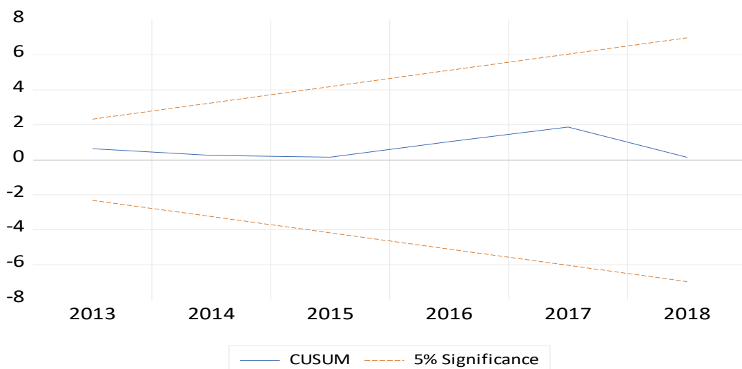
Figure 05: Plot of CUSUM test
