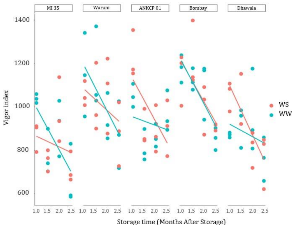
Figure 4: The effect of storage period (1, 1½, 2, and 2½ MAS - Months After Storage) on seedling vigor index (vigor index = germination percentage seedling length) of five cowpea varieties MI 35 , Waruni , Dhawala , Bombay , and ANKCP 01 . The seeds were produced under two watering treatments (well-watered-WW (-30 kPa) and water-stressed-WS (-50 kPa)) applied during their early reproductive phase.
