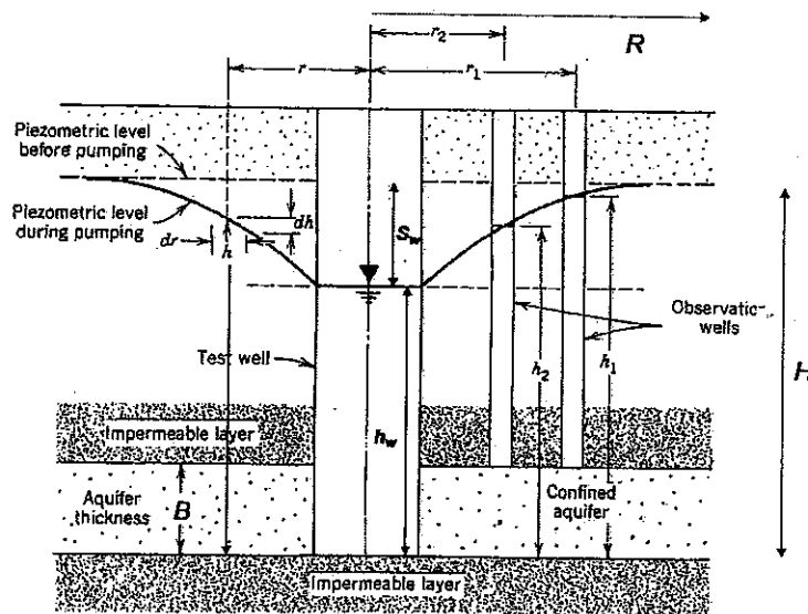
Figure Q2: Well operating in a confined aquifer
