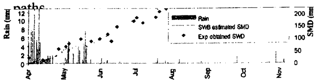
Fig.6. Experimental soil moisture deficit and soil water balance model estimated soil moisture deficit
