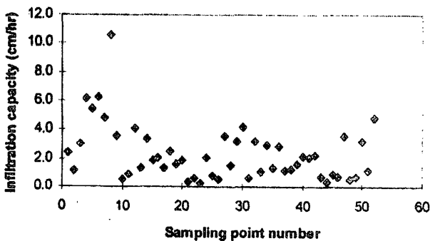
Fig.3. Infiltration capacity of surface soils at all the locations (Source ; de Silva 1996)
