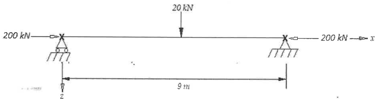
Fig. Q3(a): Bending about y-y axis
