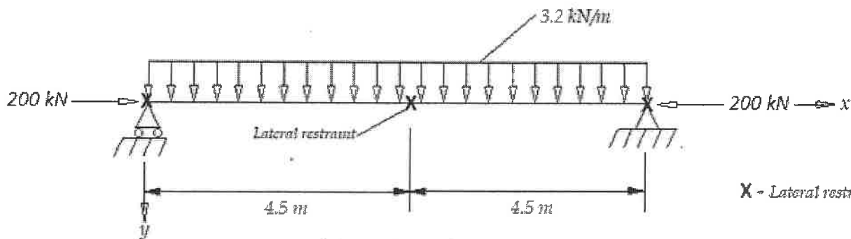
Fig. Q3(b): Bending about z-z axis
