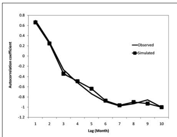
Fig. 5 - Monthly autocorrelation for observed and simulated precipitation.
