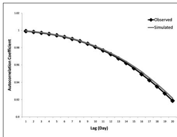
Fig. 11 - 20 days of lagged autocorrelation for observed and simulated minimum temperature.
