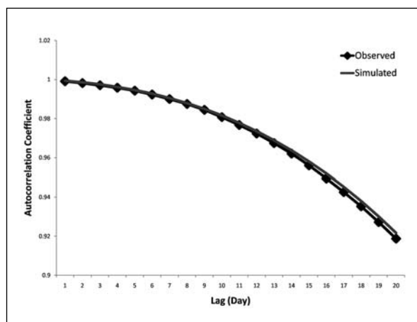
Fig. 10 - 20 days of lagged autocorrelation for observed and simulated maximum temperature.
