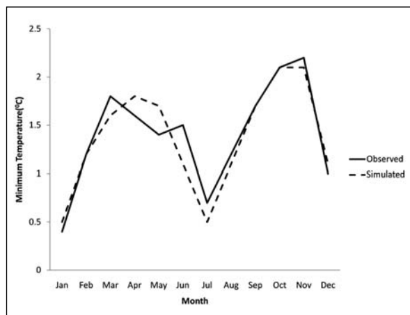
Fig. 9 - Comparison of observed and simulated standard deviation of monthly minimum temperature.
