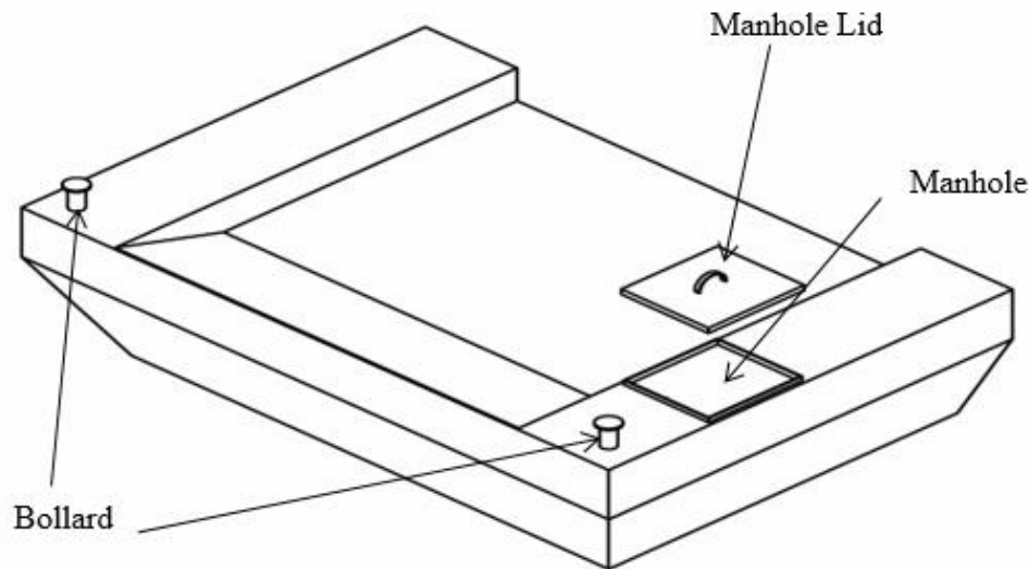
Figure 08: Bollard, Manhole and Manhole Lid
