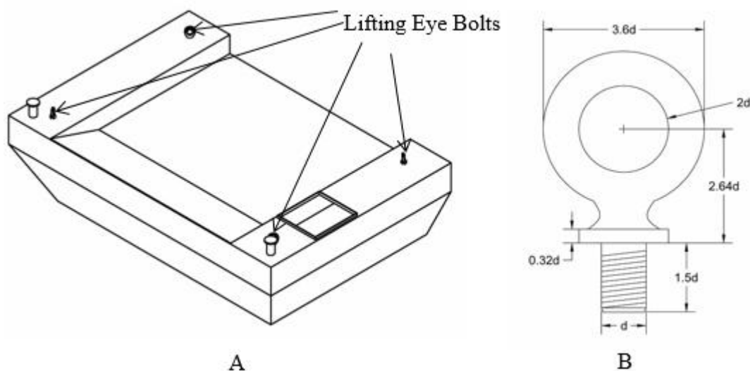
Figure 07: Lifting Eye Bolts for use to lift the piece of barge
