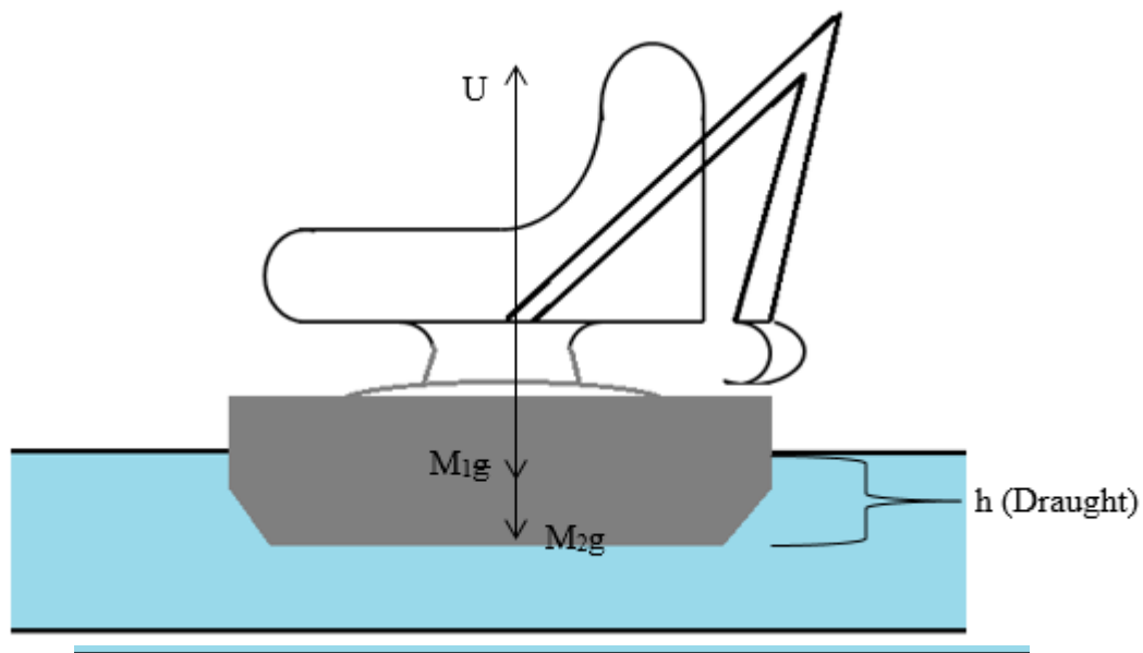
Figure 01: Force Application of the Barge and Excavator
