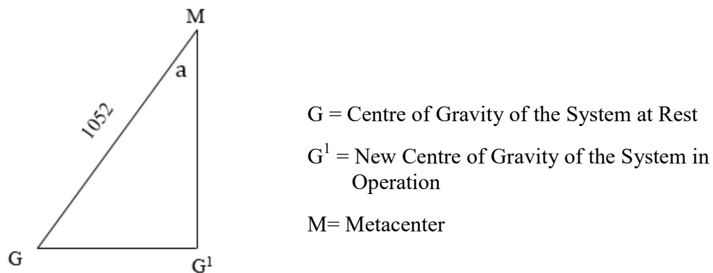
Figure 04: Triangle of the M, G and G 1
