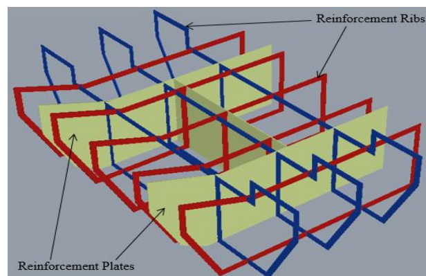
Figure 05: Reinforcement of the barge
