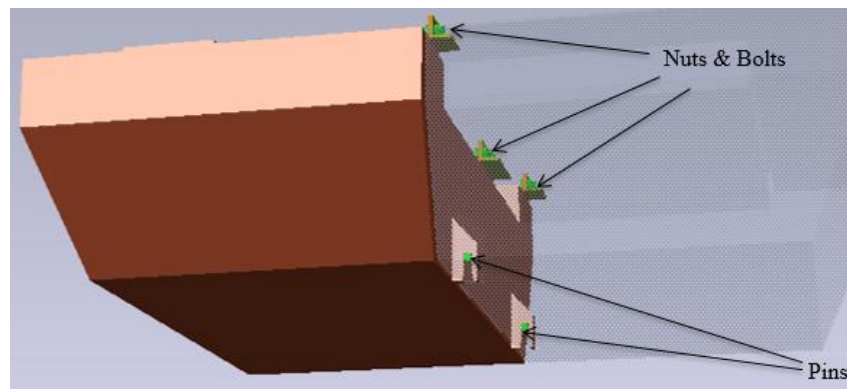
Figure 06: Nuts, Bolts and Pins used to connect of the two parts of the barge
