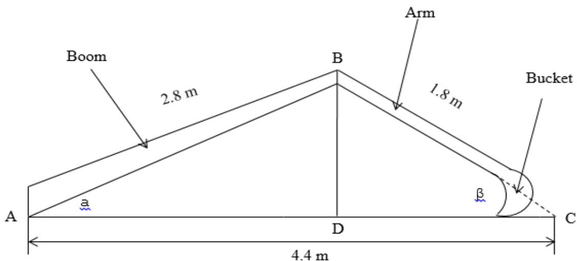
Figure 03: Geometric Representation of the Boom, Arm and Bucket
